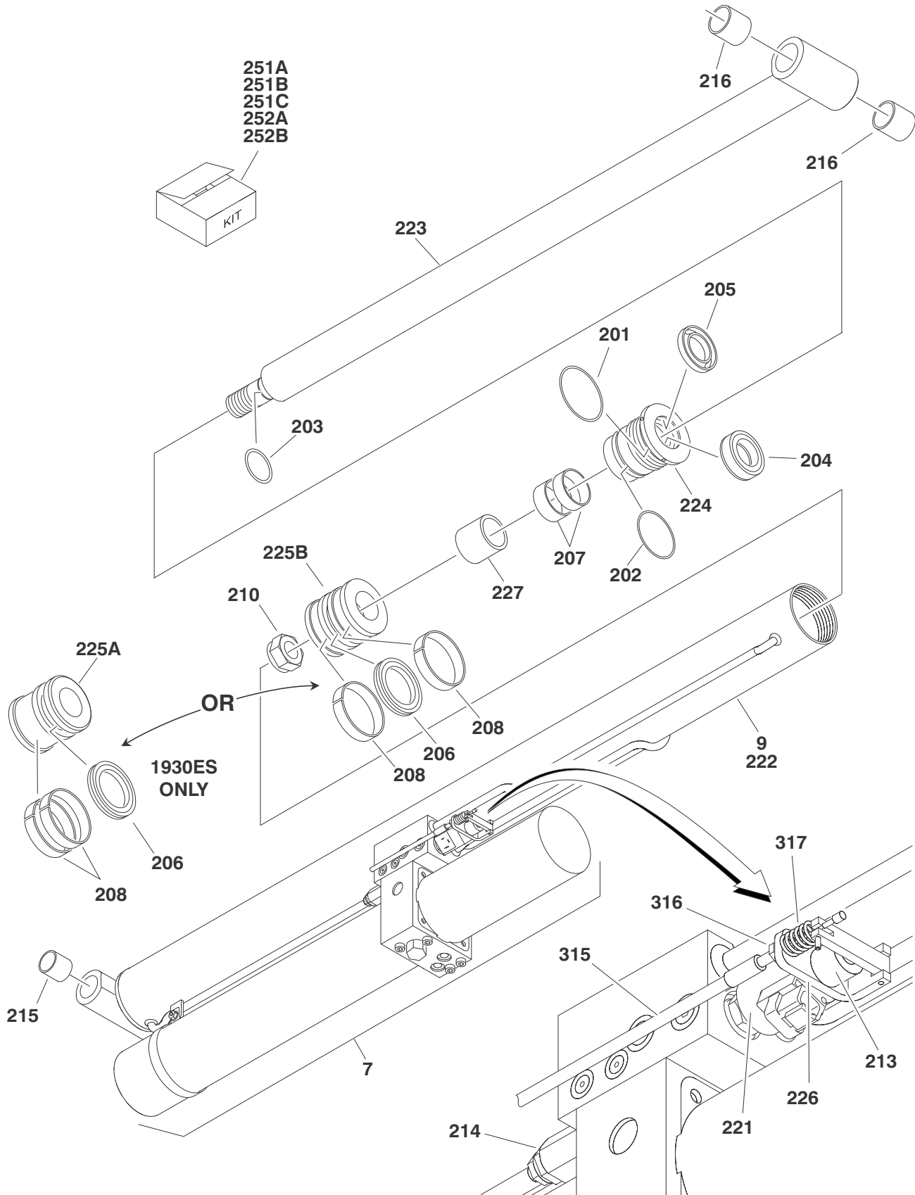
FIGURE 5-1.LIFT CYLINDER ASSEMBLY (TEXAS HYDRAULICS)
