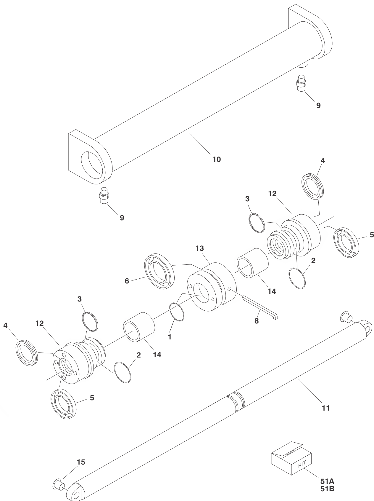
FIGURE 5-3. STEER CYLINDER ASSEMBLY (TEXAS HYDRAULICS)
