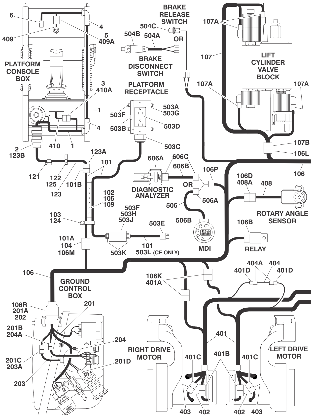
FIGURE 7-3. 2646ES/3246ES ELECTRICAL COMPONENTS INSTALLATION
