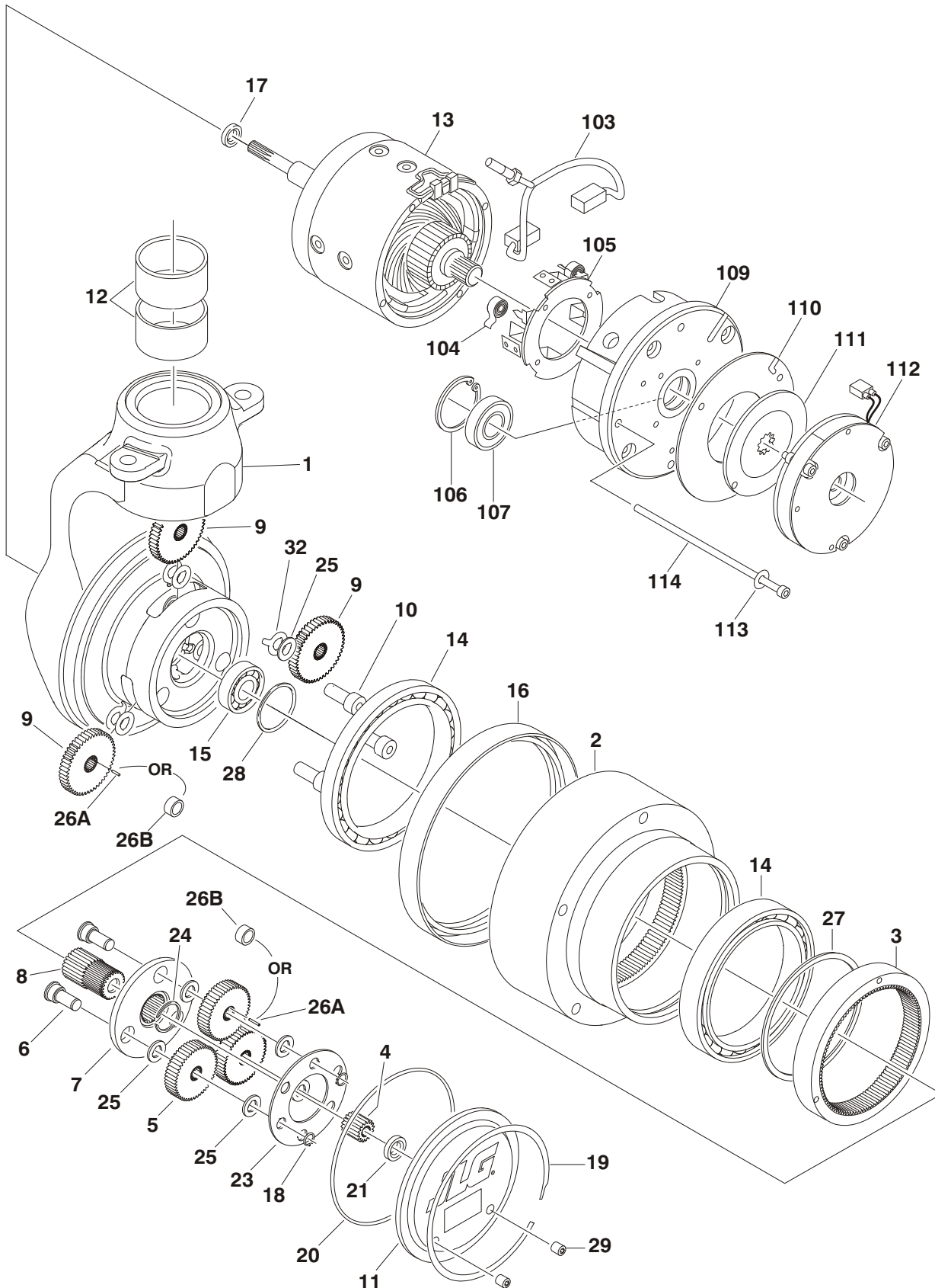
FIGURE 1-2.WHEEL DRIVE ASSEMBLY
