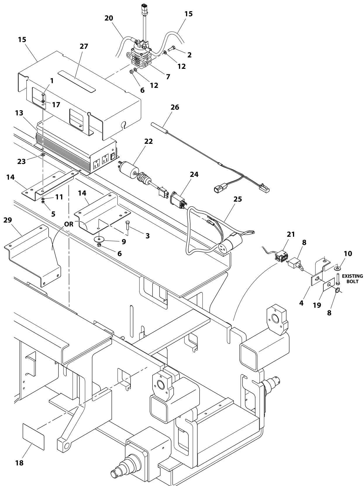
FIGURE 1-8. INVERTER INSTALLATION (WITHOUT BATTERY CHARGER) (OPTIONAL ON ANSI SPEC MACHINES)
