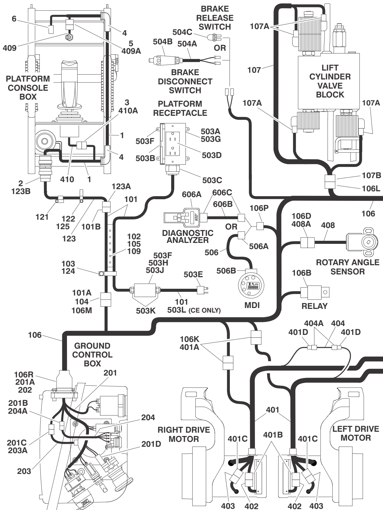
FIGURE 7-2. 2030ES/2630ES ELECTRICAL COMPONENTS INSTALLATION
