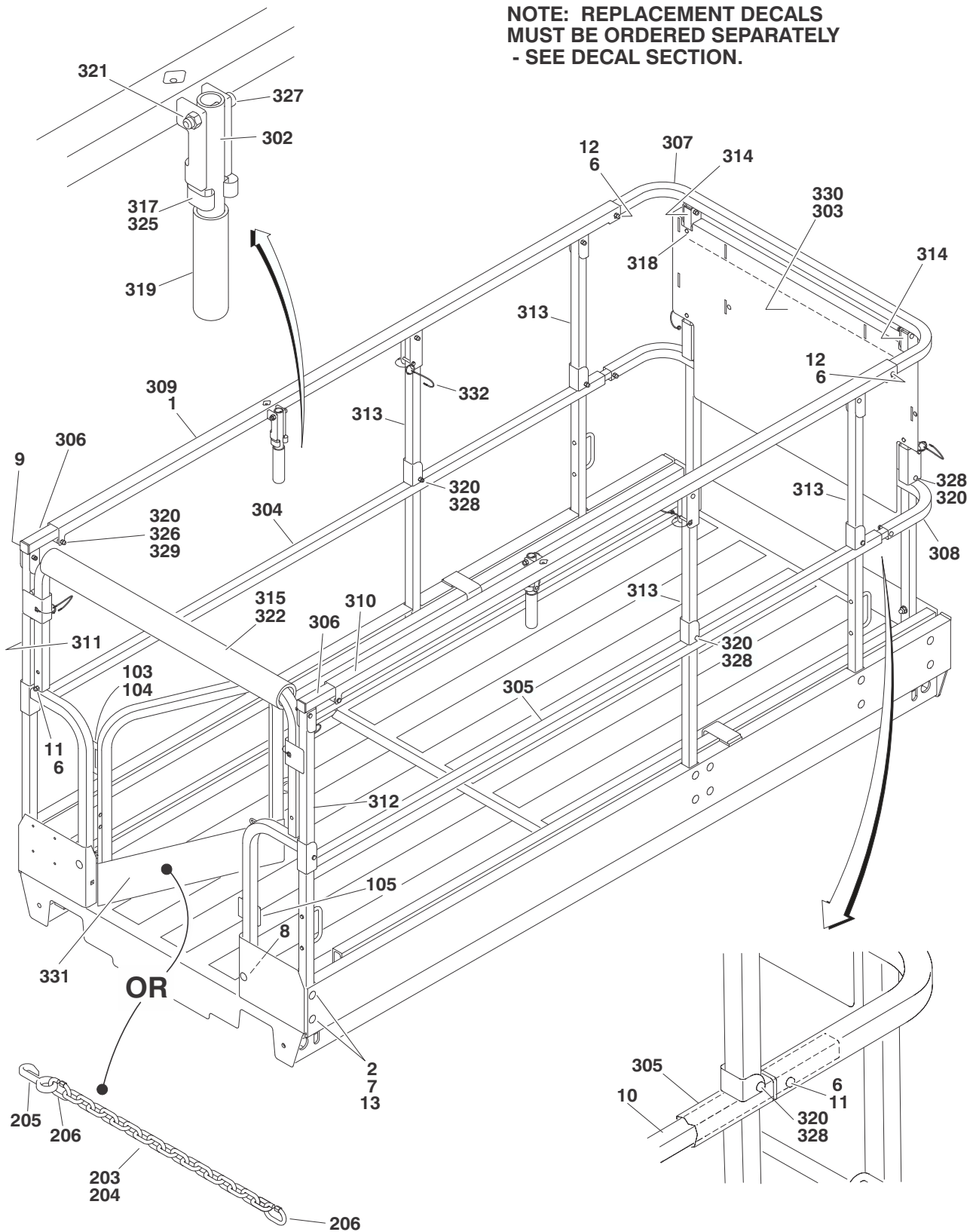
FIGURE 4-5.RAIL INSTALLATION - 2646ES/3246ES
