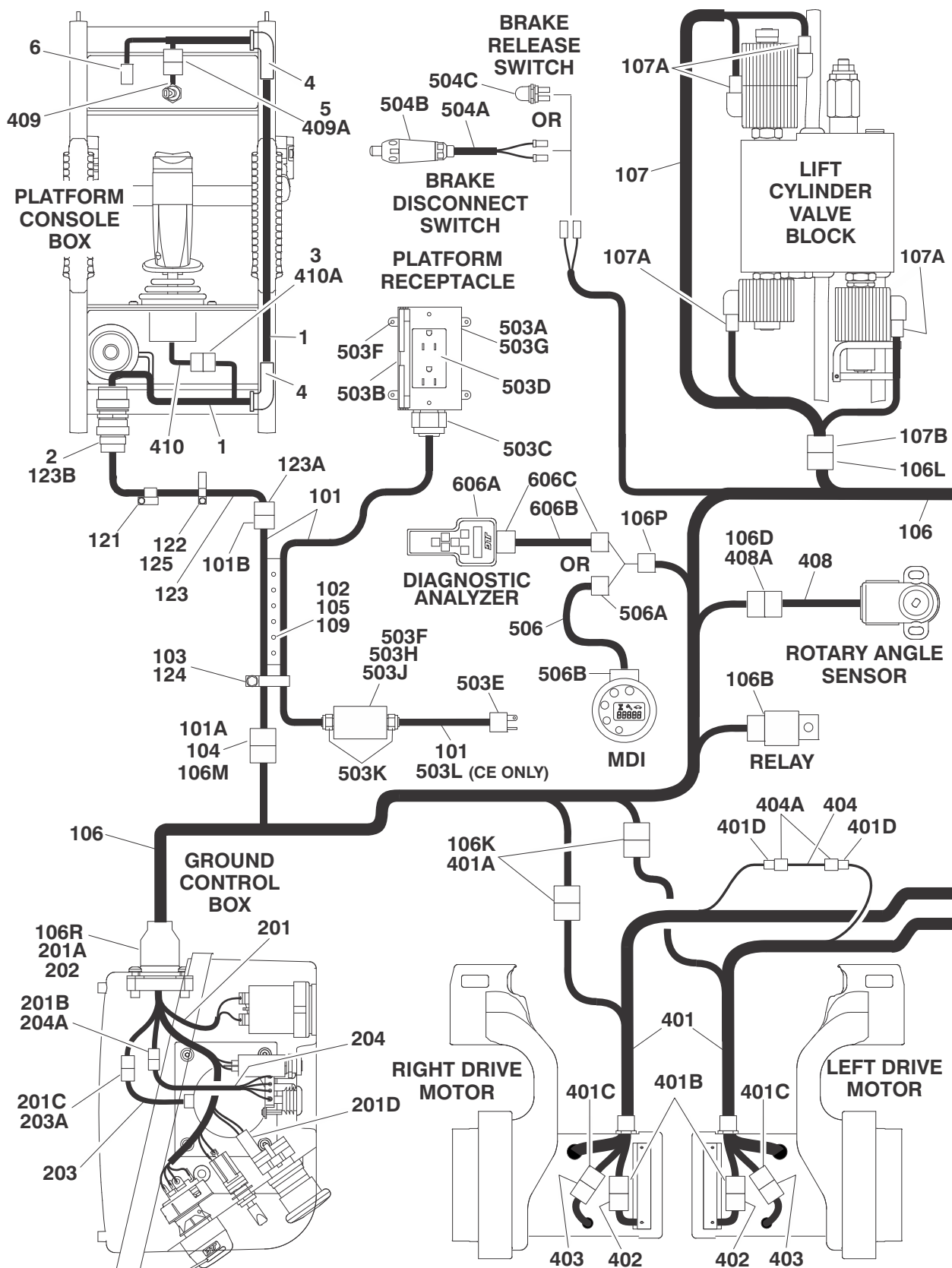
FIGURE 7-1. 1930ES ELECTRICAL COMPONENTS INSTALLATION
