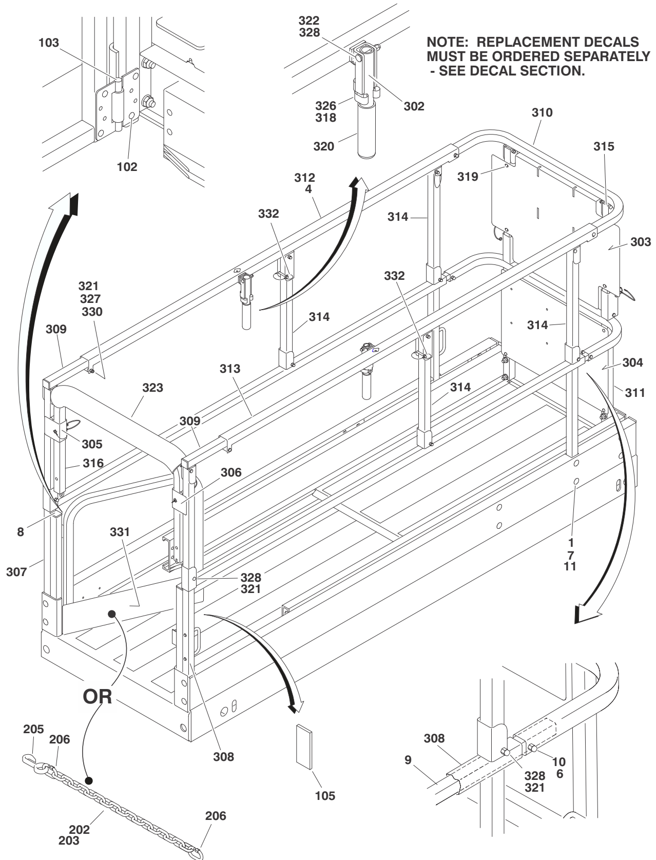
FIGURE 4-4.RAIL INSTALLATION - 2030ES/2630ES
